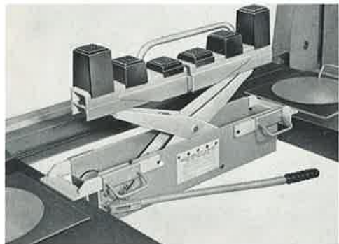
792 JACKING BEAM 1 tonne.
