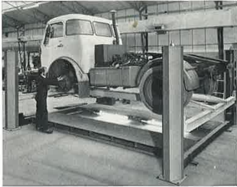
788 A 'Dockmaster' 4 post 'Tractor' Unit lift 8 tonnes.
